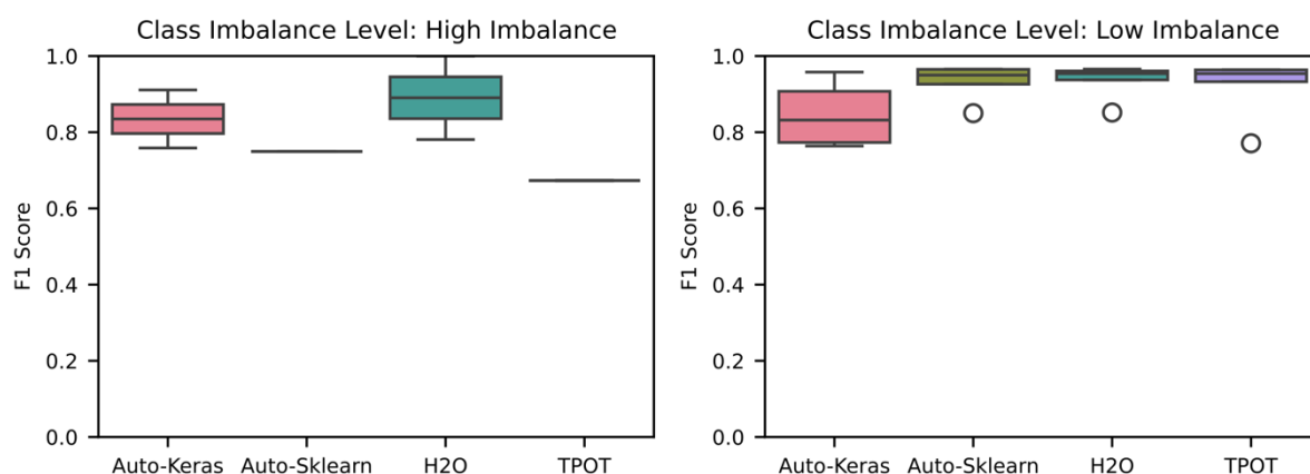
Figure 2. Multiclass classification results.
